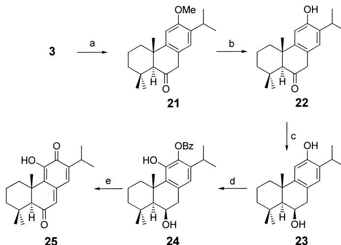
Scheme 4. (a) (i) mCPBA, \text{CHCl}_3 , 3 – 8^\circ\text{C} , 4.5 h; (ii) TsOH, \text{CHCl}_3 , reflux, 2 h, two steps, 61.4%; (b) \text{BBr}_3 , \text{CH}_2\text{Cl}_2 , 20^\circ\text{C} , 2.5 h, 60.6%; (c) \text{LiAlH}_4 , THF, reflux, 1 h, 80.2%; (d) BPO, \text{CHCl}_3 , 35^\circ\text{C} , 48 h, 72.4%; (e) (i) \text{LiAlH}_4 , THF, reflux, 1.5 h; (ii) Jones' reagent, acetone, 0^\circ\text{C} , 5 min, two steps, 97.9%.
